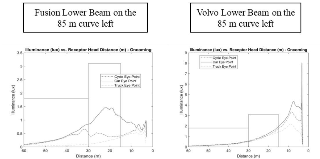
Figure 14. Lower beam performance on 85 m Left curve
