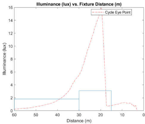
ADB Radius 85 m Left motorcycle fixture (Lexus ADB at 26 mph)
