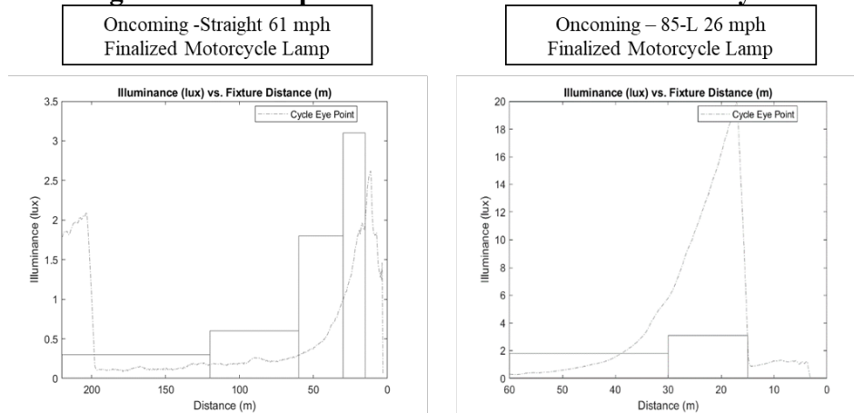
Figure C.1. ADB performance with final rule motorcycle fixture
