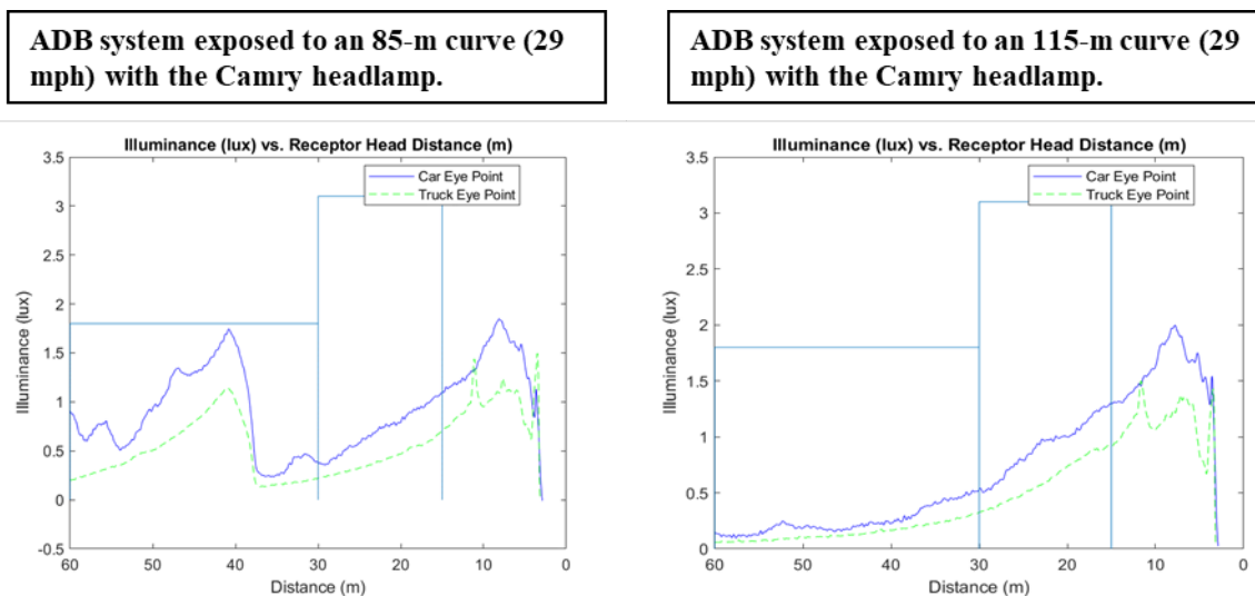
Figure 2. ADB system with oncoming car/truck fixture on left curve, R85 m vs. R115 m
