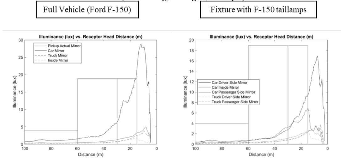
Figure 5. ADB performance with stimulus vehicle vs. stimulus fixture (Preceding, straight, 69 mph)
