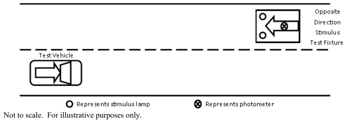
Figure 27 Opposite Direction Test Scenarios
