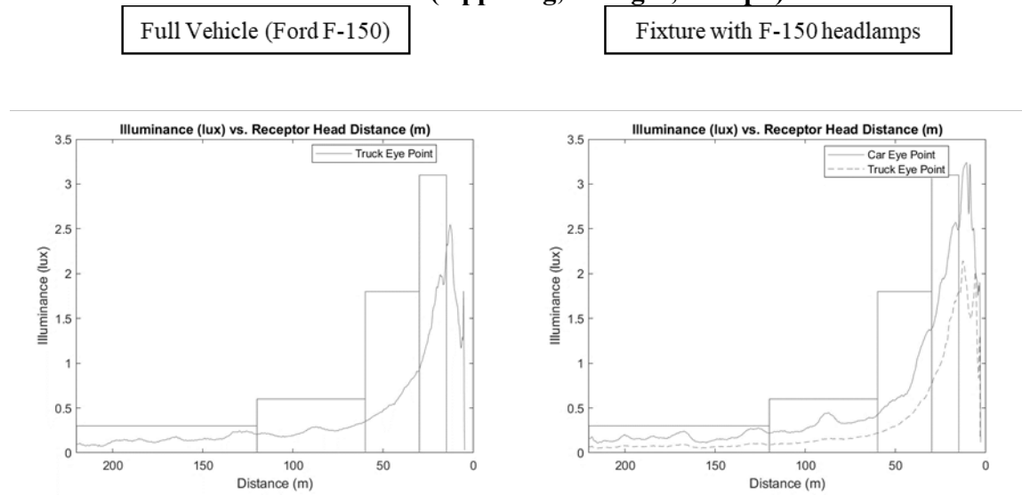
Figure 4. ADB performance with stimulus vehicle vs. stimulus fixture (Opposing, Straight, 69 mph)
