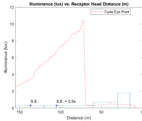
SAE Motorcycle Fixture, Position 1, Sudden appearance (Lexus ADB at 28 mph)
