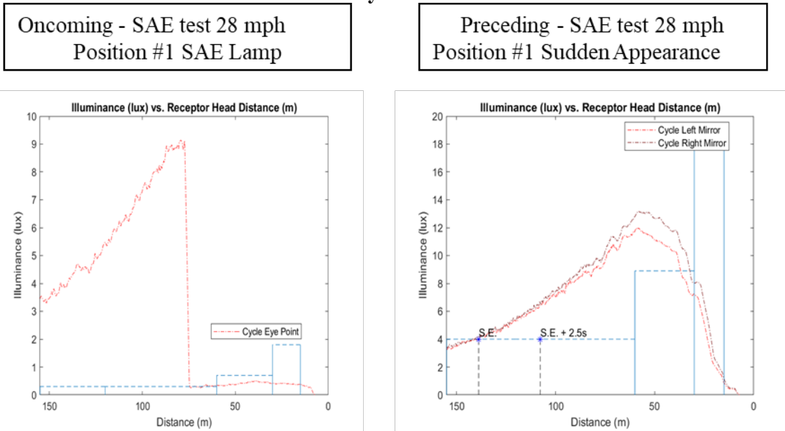
Figure C.3. Examples of ADB failures when tested against the SAE J3069 motorcycle fixtures
