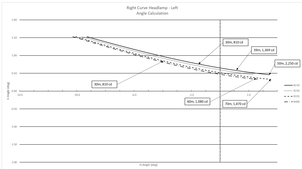
Figure A.1. Horizontal angle for each headlamp (right and left) at each extreme of each right curve
