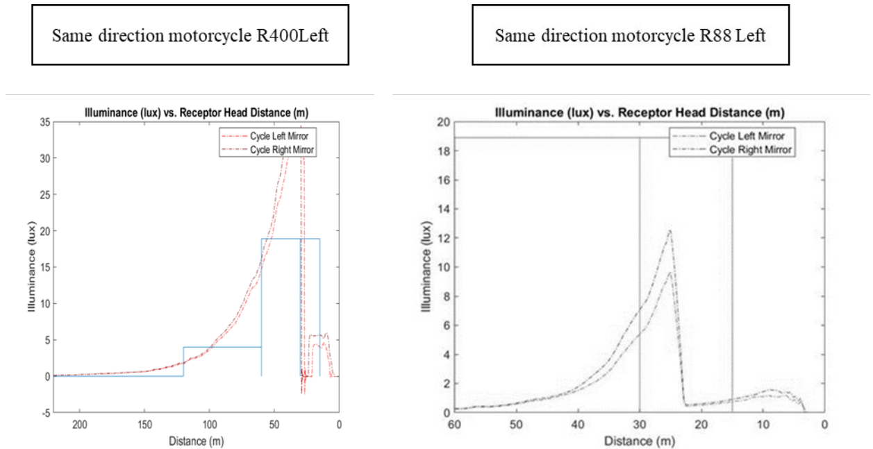
Figure 3. ADB system with preceding motorcycle fixture on left curve (R400 and R88)
