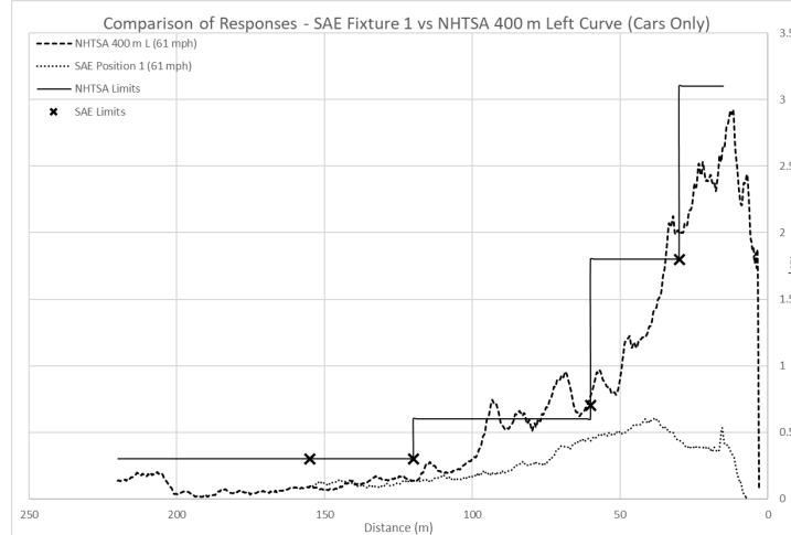
Figure 22. SAE test vs. large oncoming curve scenario
