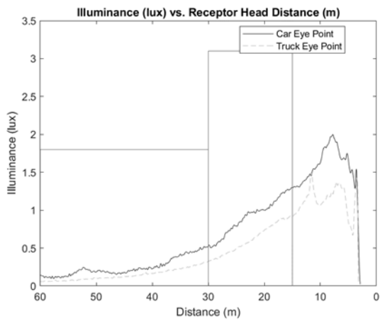
Figure 15 - Lexus ADB 29 mph on the 115-m curve Left (Camry HL)
