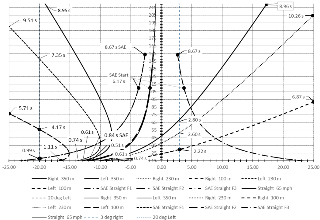
Figure 7. Comparison of fixture trajectories in SAE J3069 and final rule
